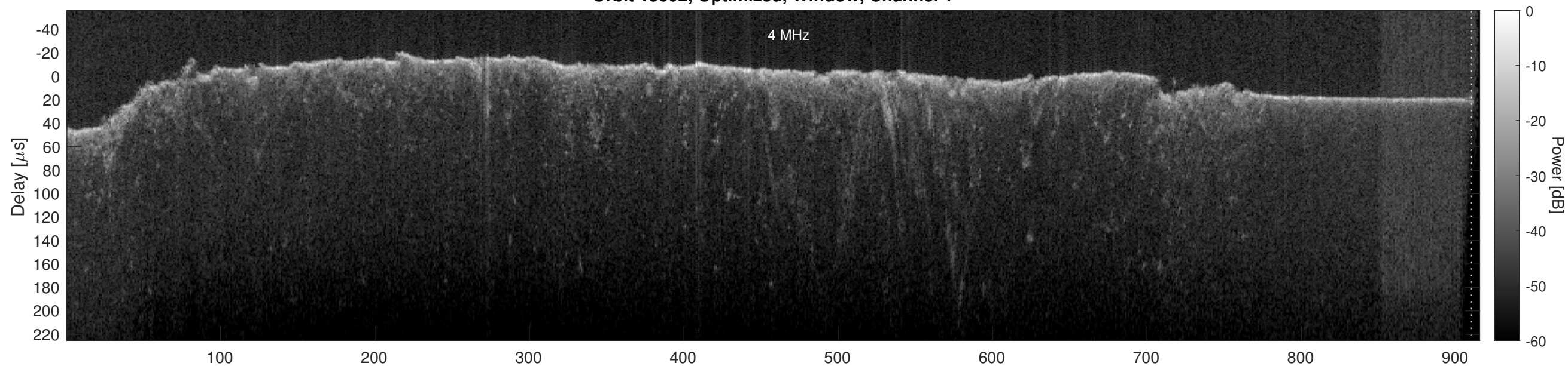
Orbit 18602, Optimized, Window, Channel 2
