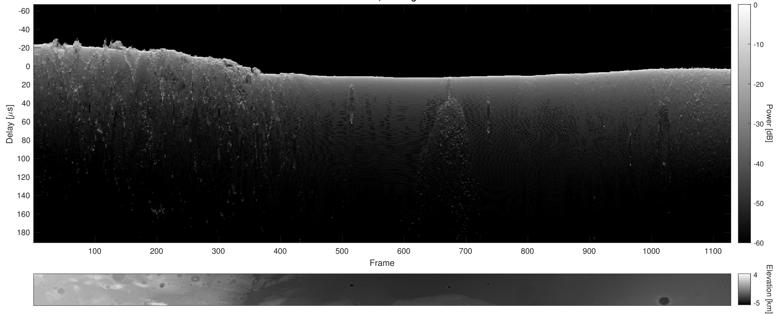
Orbit 18604, Cluttergram
