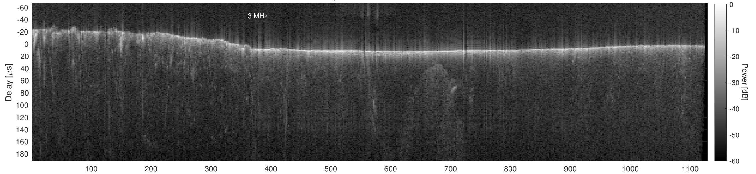
Orbit 18604, Cluttergram
