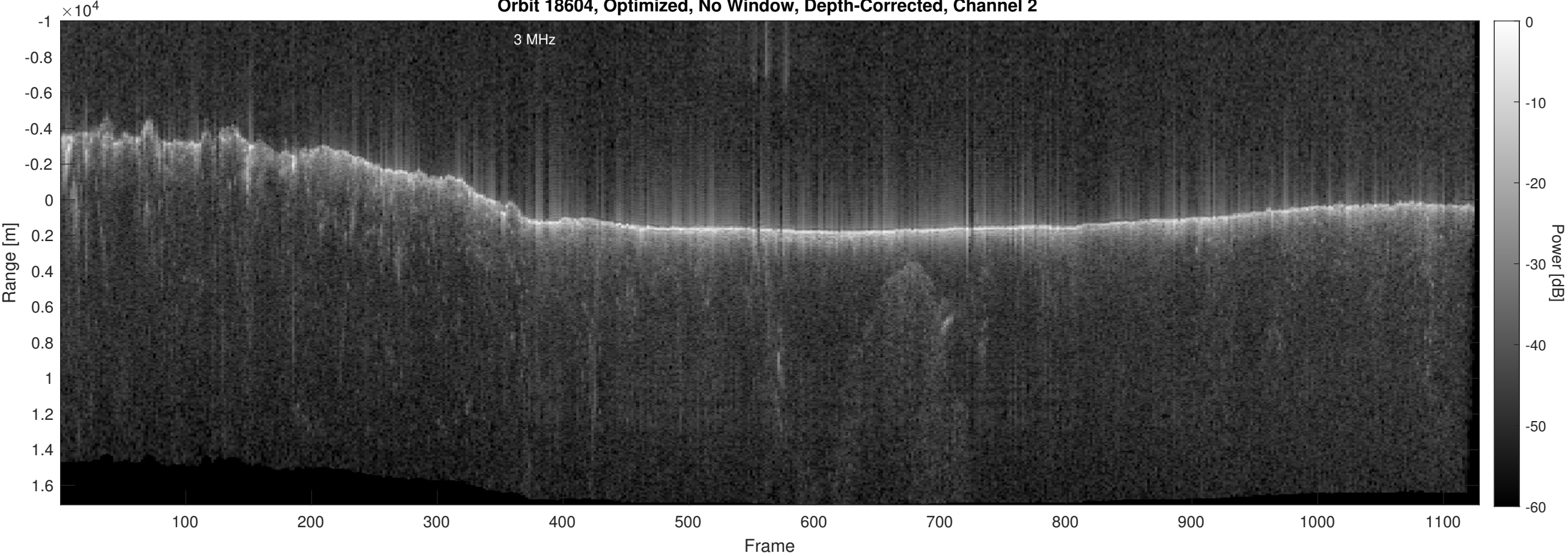
Orbit 18604, Optimized, No Window, Depth-Corrected, Channel 2
