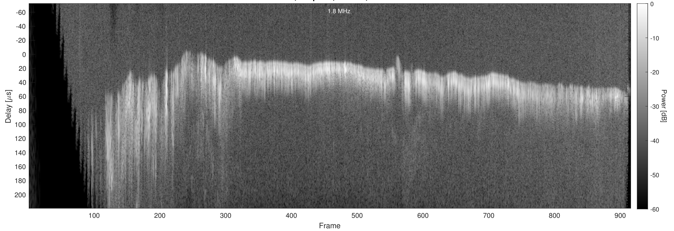
Orbit 18607, Chapman, Window, Channel 2
