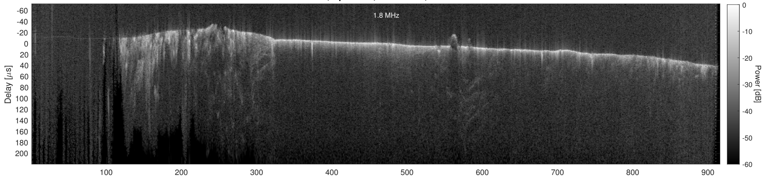
Orbit 18607, Cluttergram
