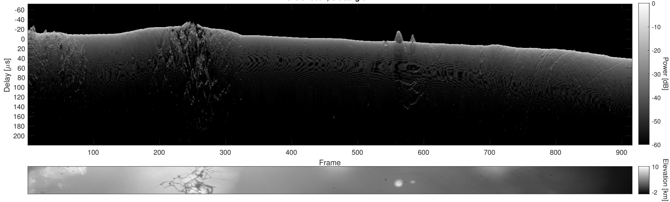
Orbit 18607, Cluttergram
