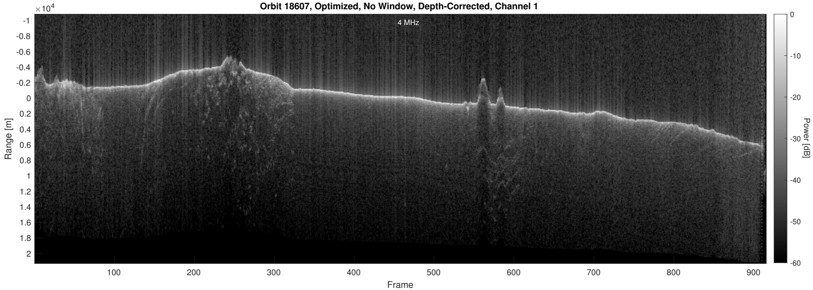
Orbit 18607, Optimized, No Window, Depth-Corrected, Channel 2
