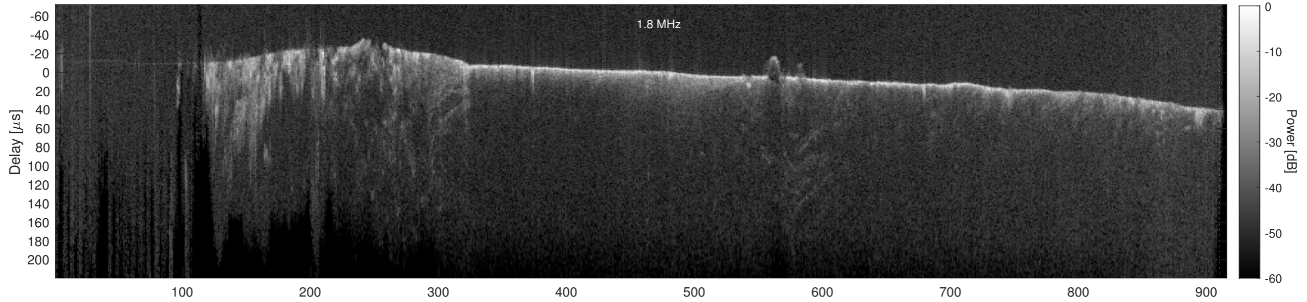
Orbit 18607, Cluttergram
