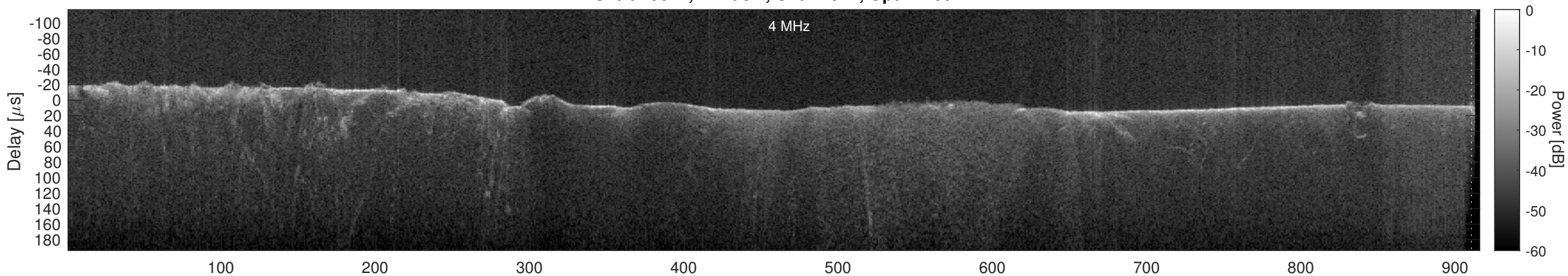
Orbit 18611, Cluttergram
