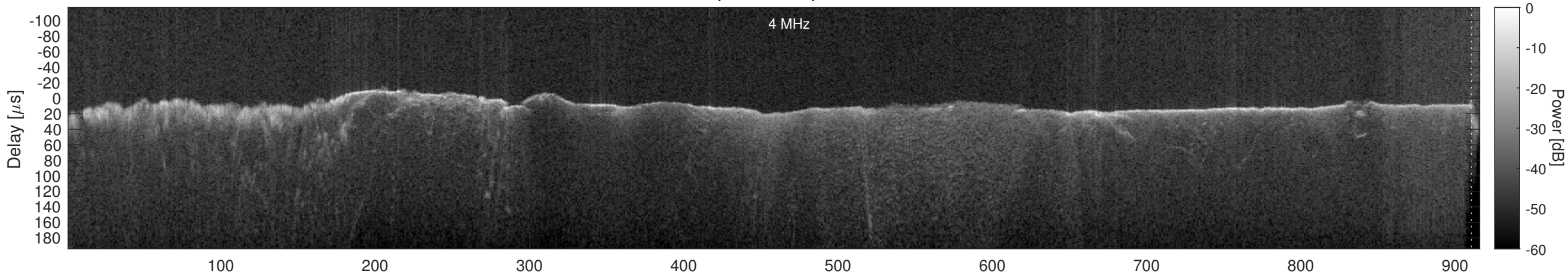
Orbit 18611, Window, Channel 1, Chapman
