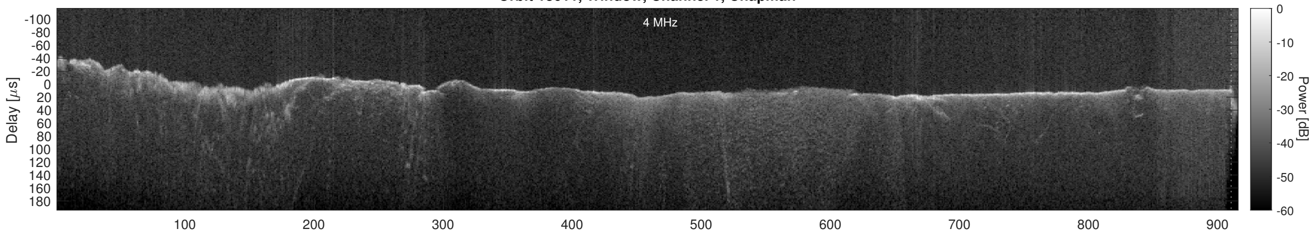
Orbit 18611, Window, Channel 1, Optimized
