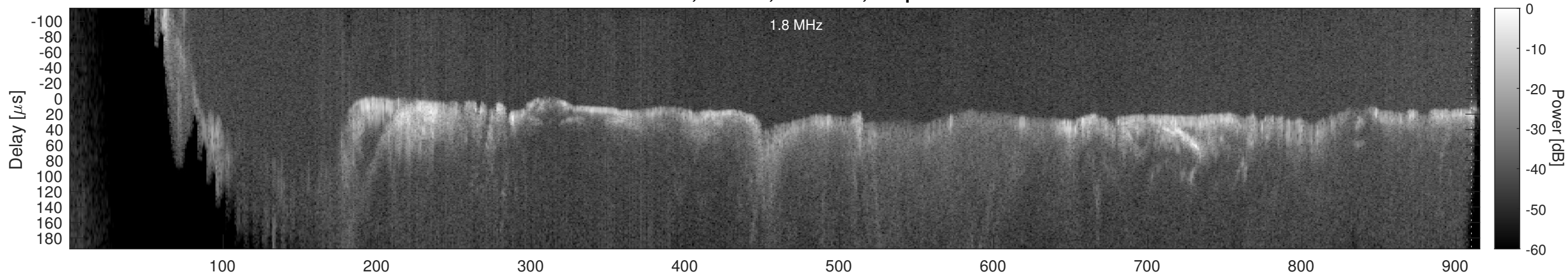
Orbit 18611, Window, Channel 2, Optimized
