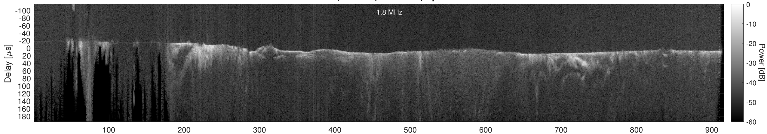
Orbit 18611, Cluttergram
