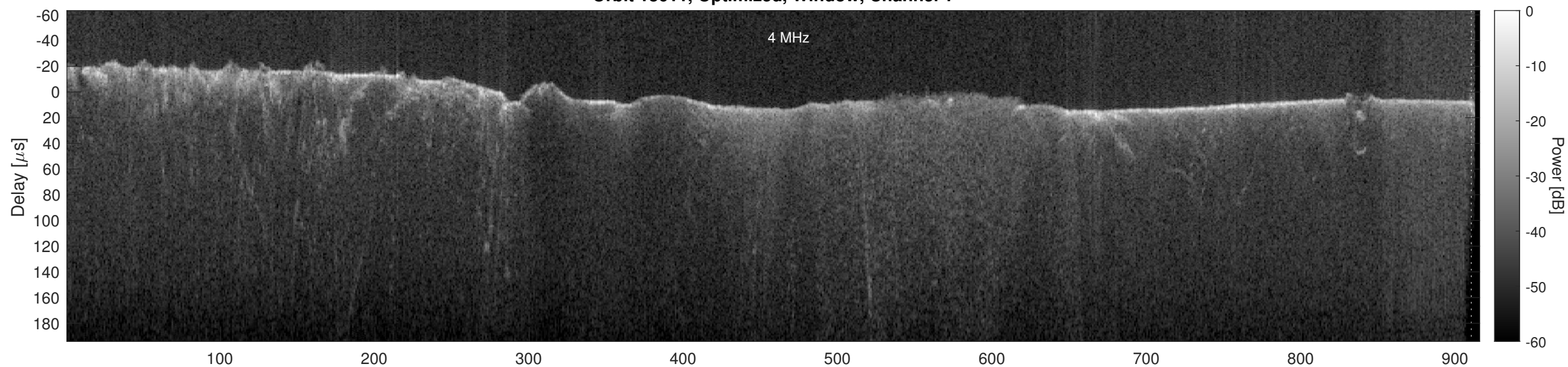
Orbit 18611, Optimized, Window, Channel 2
