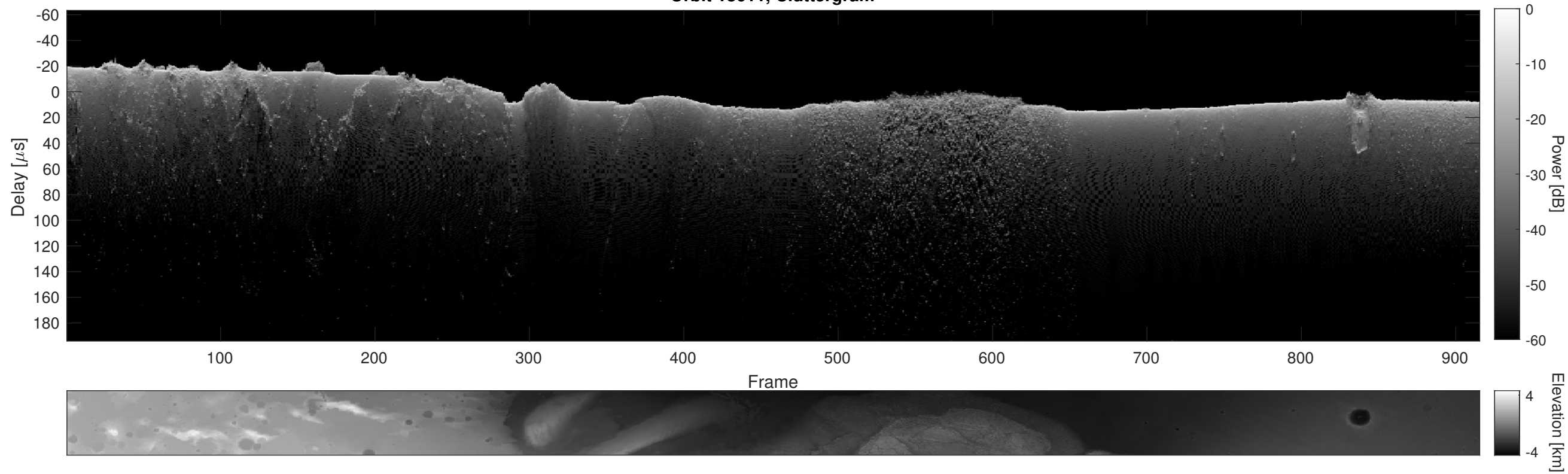
Orbit 18611, Cluttergram
