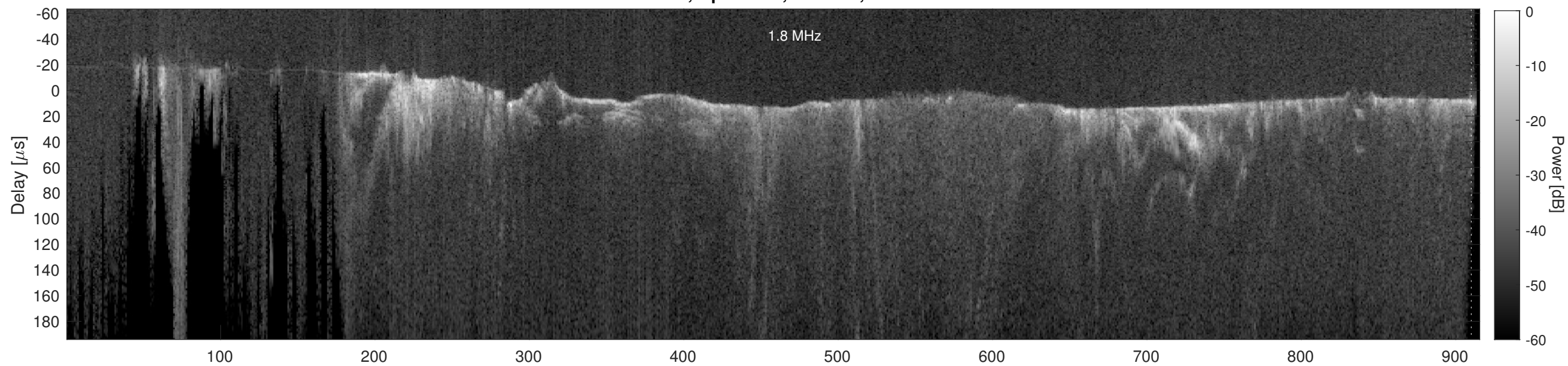
Orbit 18611, Cluttergram
