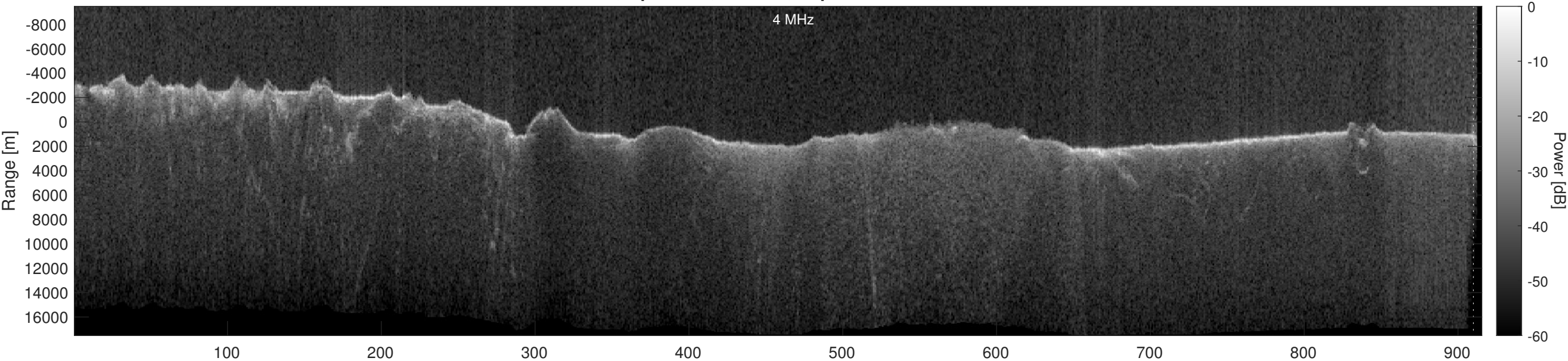
Orbit 18611, Optimized, Window, Depth-Corrected, Channel 2
