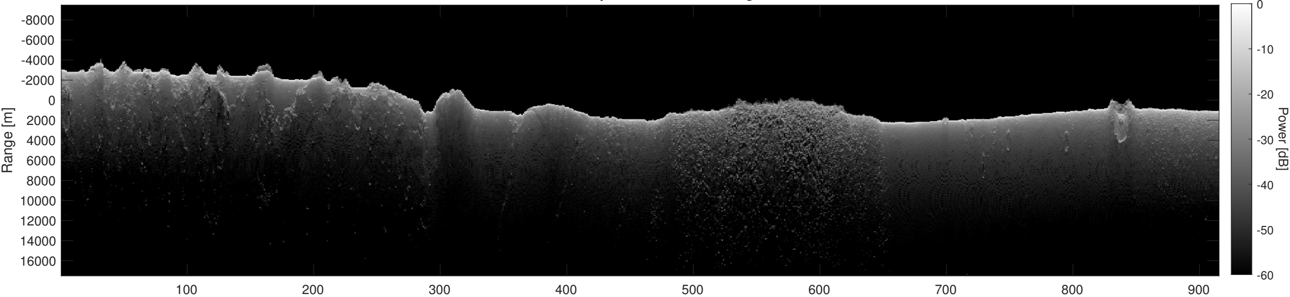
Orbit 18611, Depth-Corrected Cluttergram
