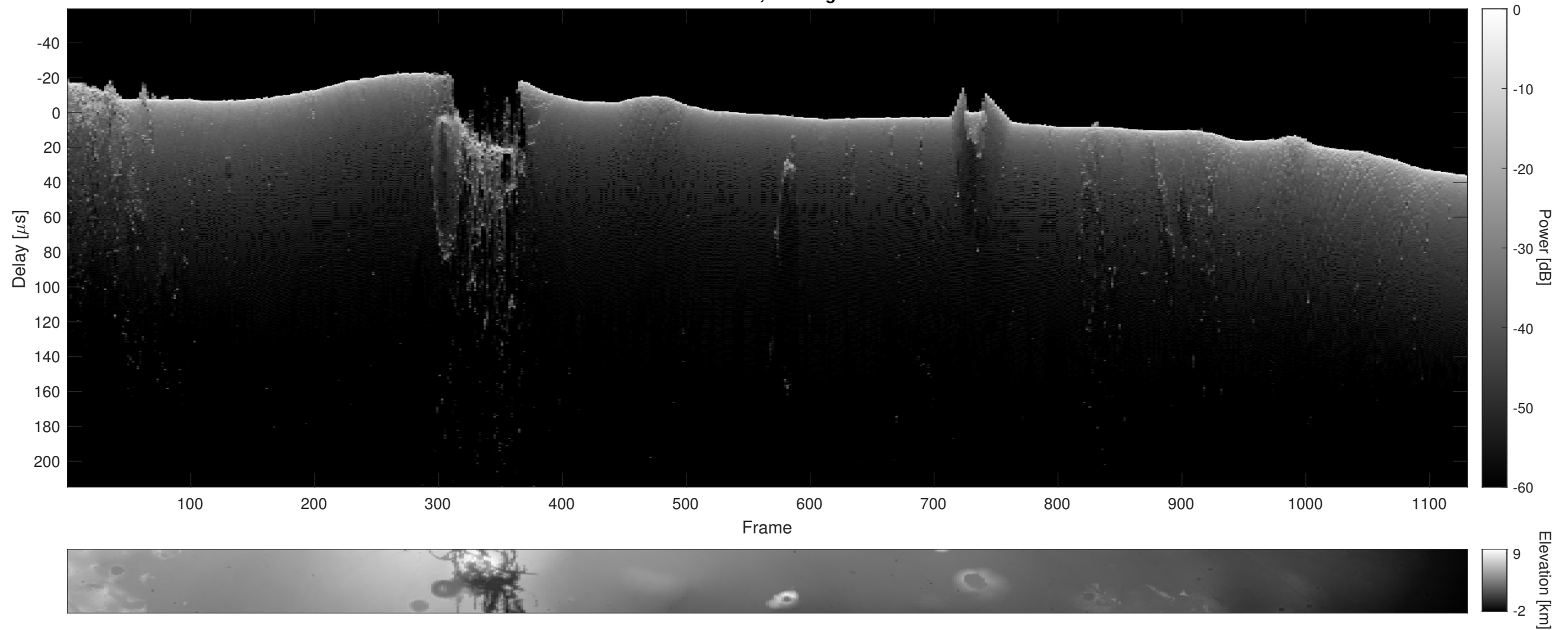
Orbit 18614, Cluttergram
