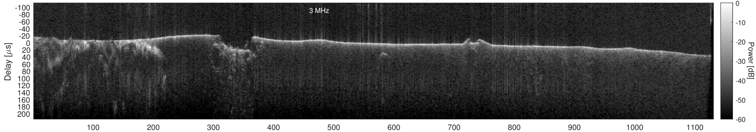
Orbit 18614, Cluttergram
