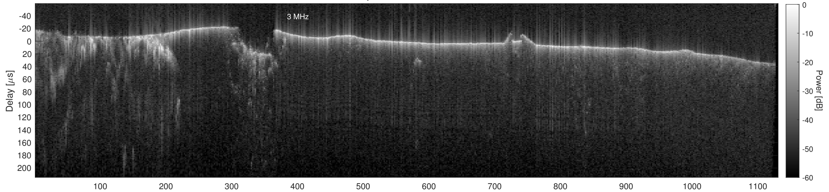
Orbit 18614, Cluttergram
