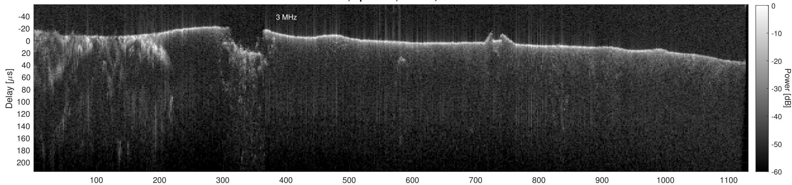
Orbit 18614, Cluttergram
