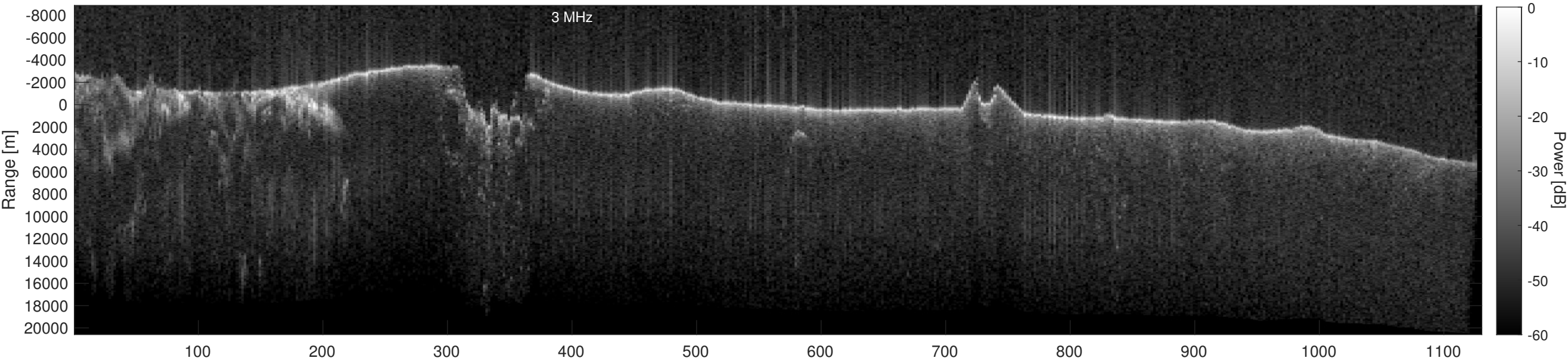
Orbit 18614, Depth-Corrected Cluttergram
