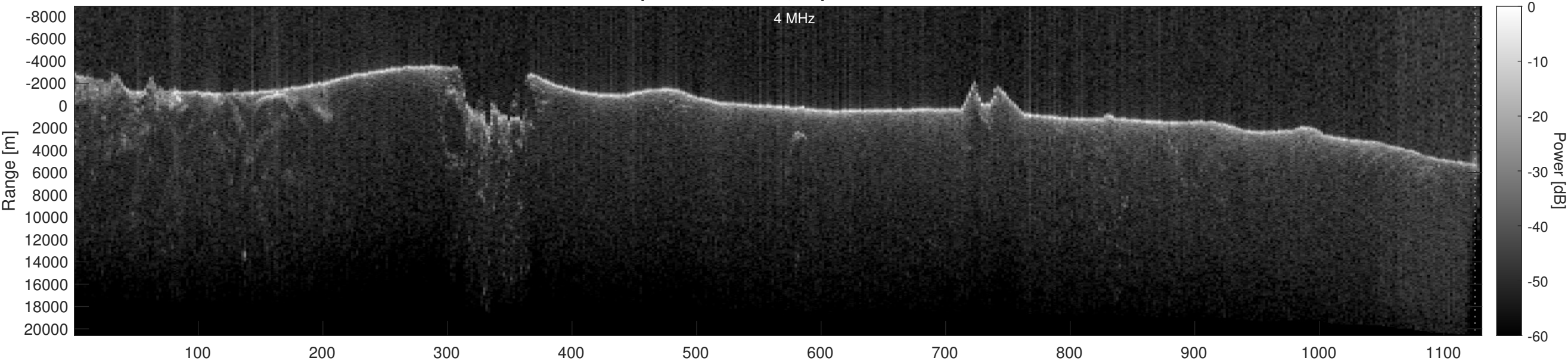
Orbit 18614, Optimized, Window, Depth-Corrected, Channel 2
