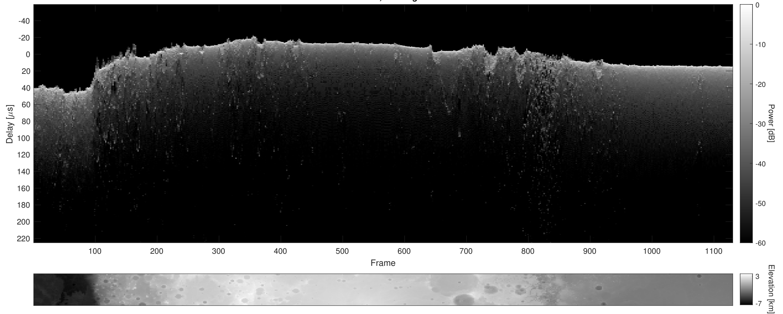
Orbit 18616, Cluttergram
