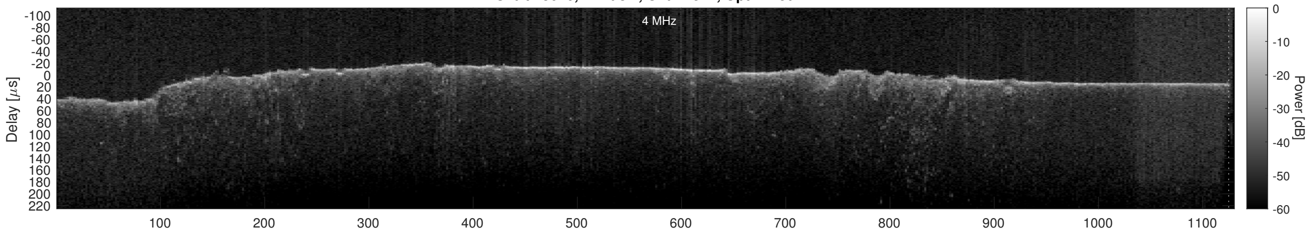
Orbit 18616, Cluttergram
