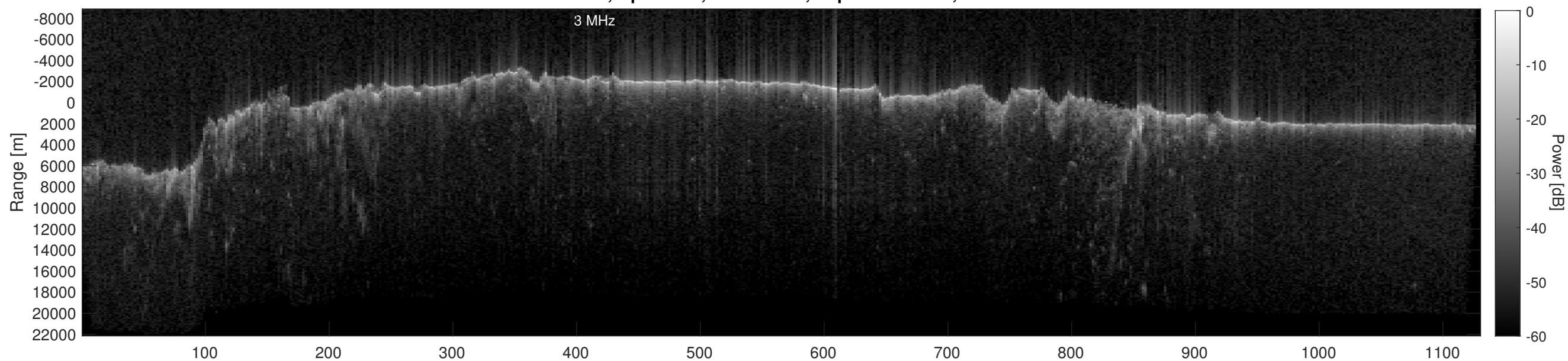
Orbit 18616, Depth-Corrected Cluttergram
