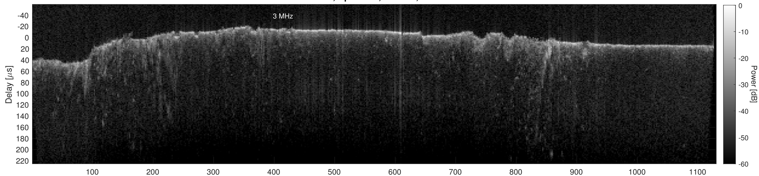
Orbit 18616, Cluttergram
