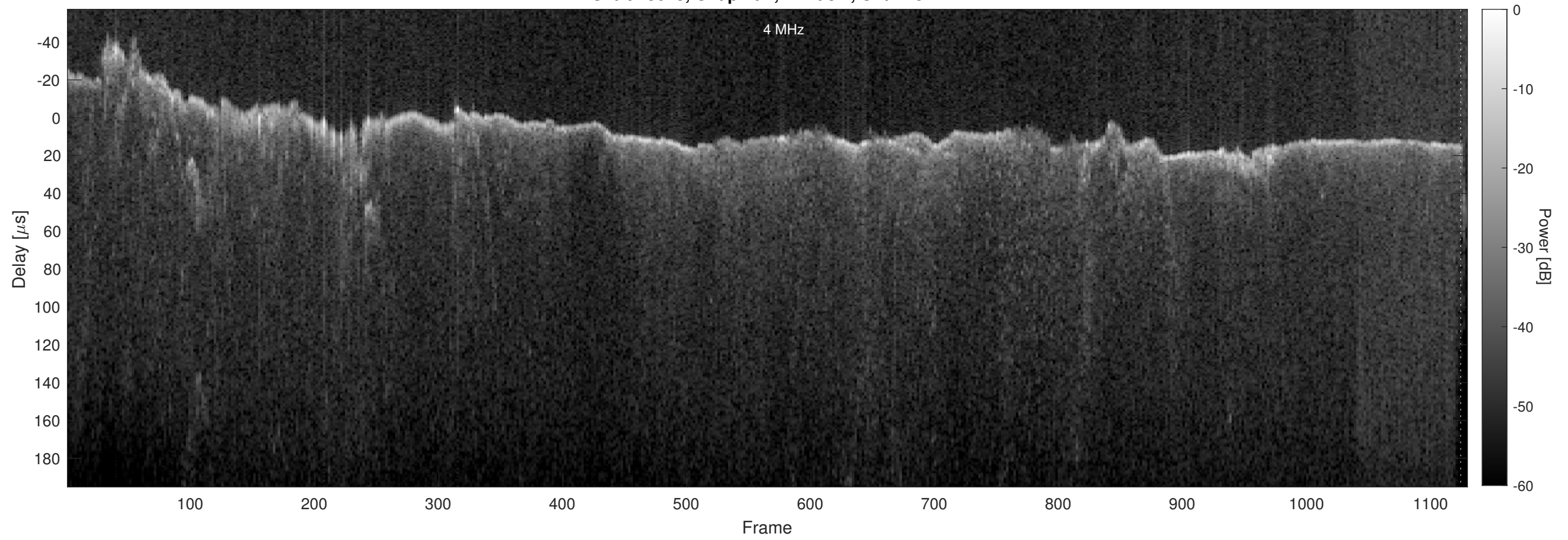
Orbit 18618, Chapman, Window, Channel 2
