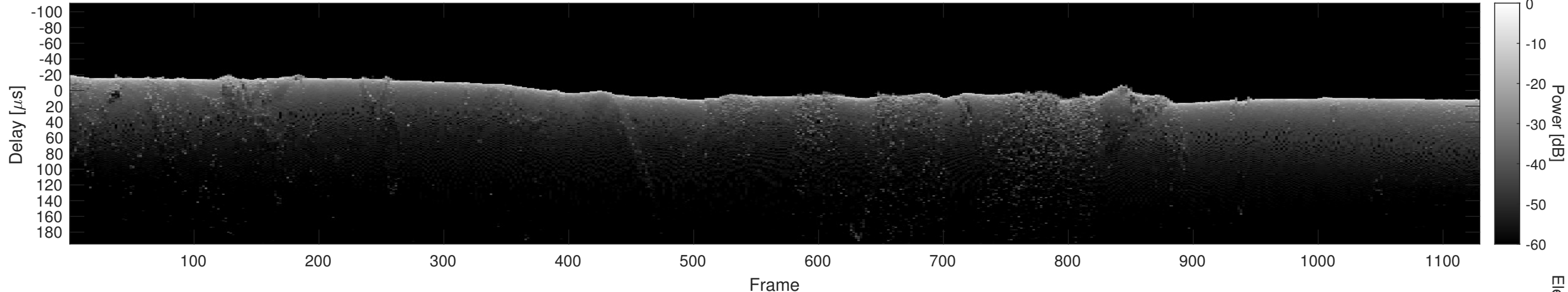
Orbit 18618, Cluttergram
