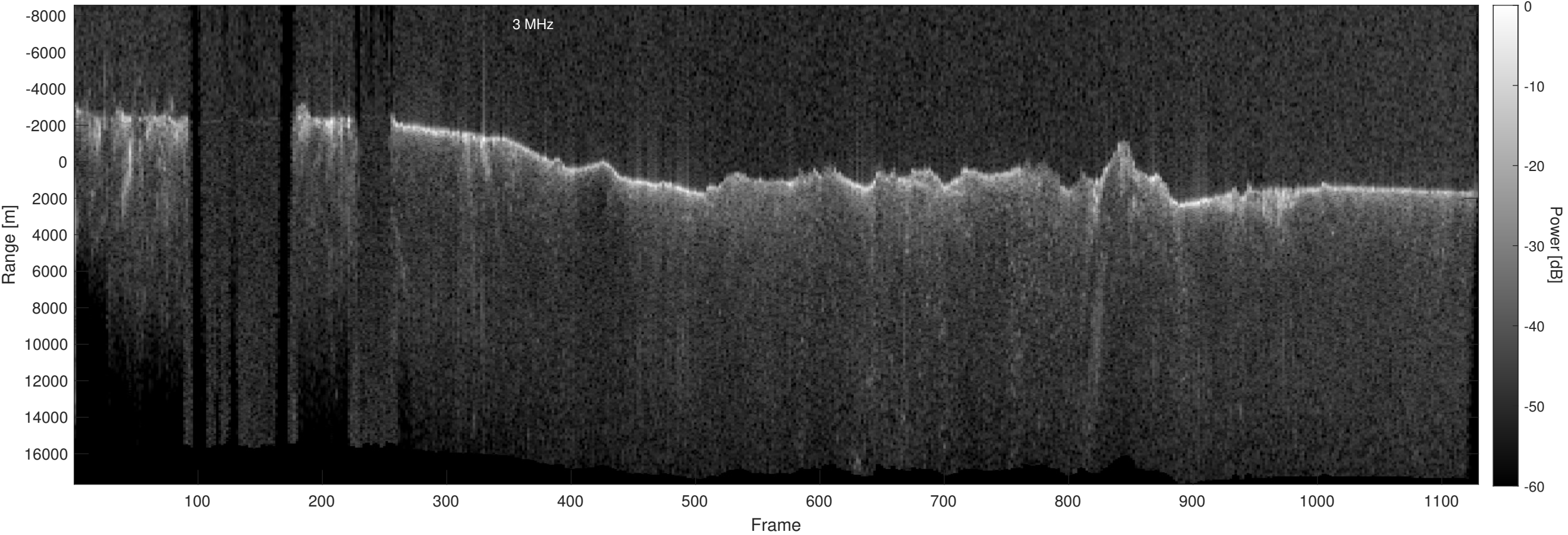
Orbit 18618, Optimized, Window, Depth-Corrected, Channel 2
