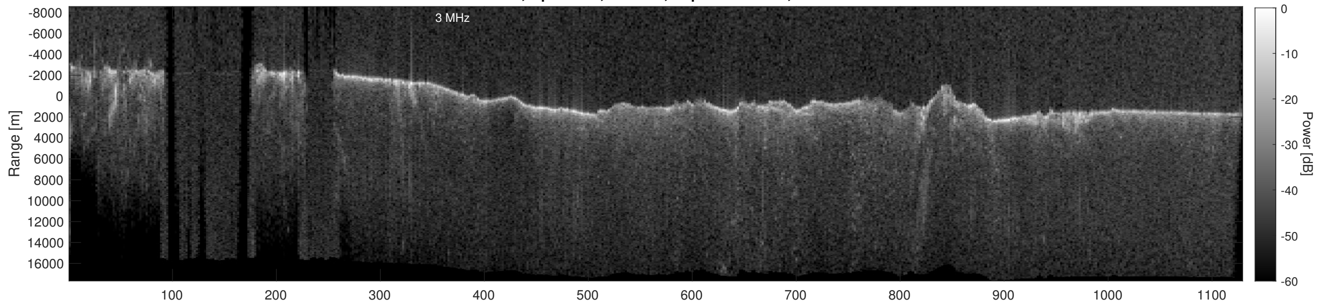
Orbit 18618, Depth-Corrected Cluttergram
