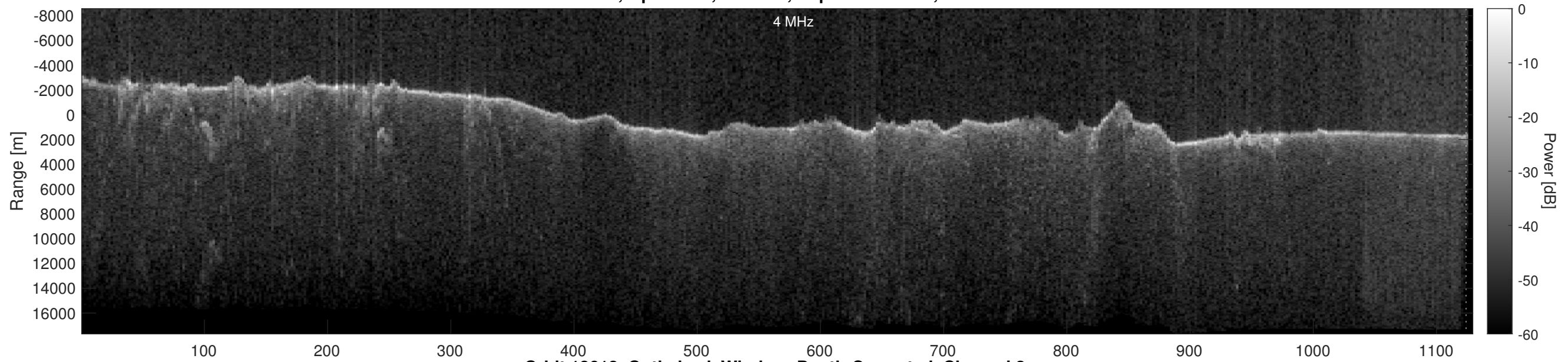
Orbit 18618, Optimized, Window, Depth-Corrected, Channel 2
