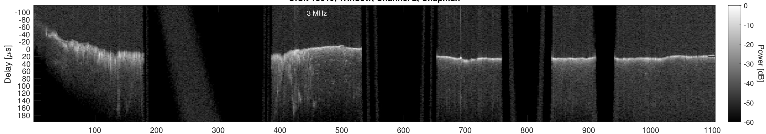
Orbit 18619, Window, Channel 2, Optimized
