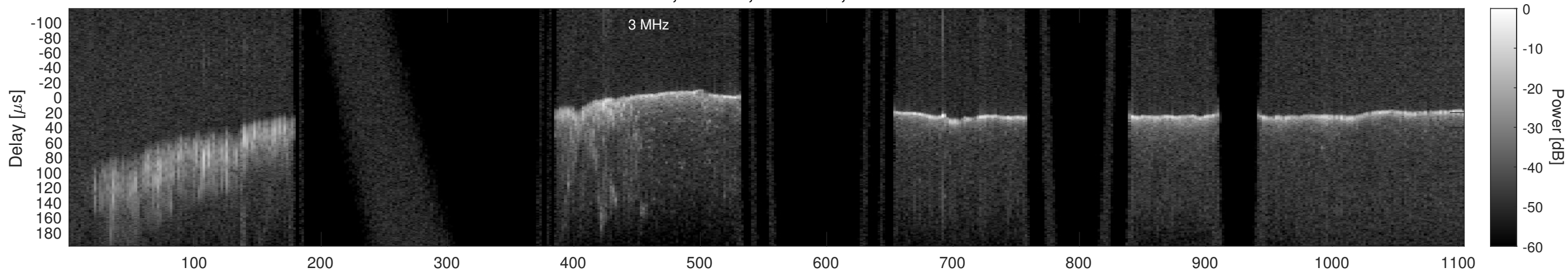
Orbit 18619, Window, Channel 2, Chapman
