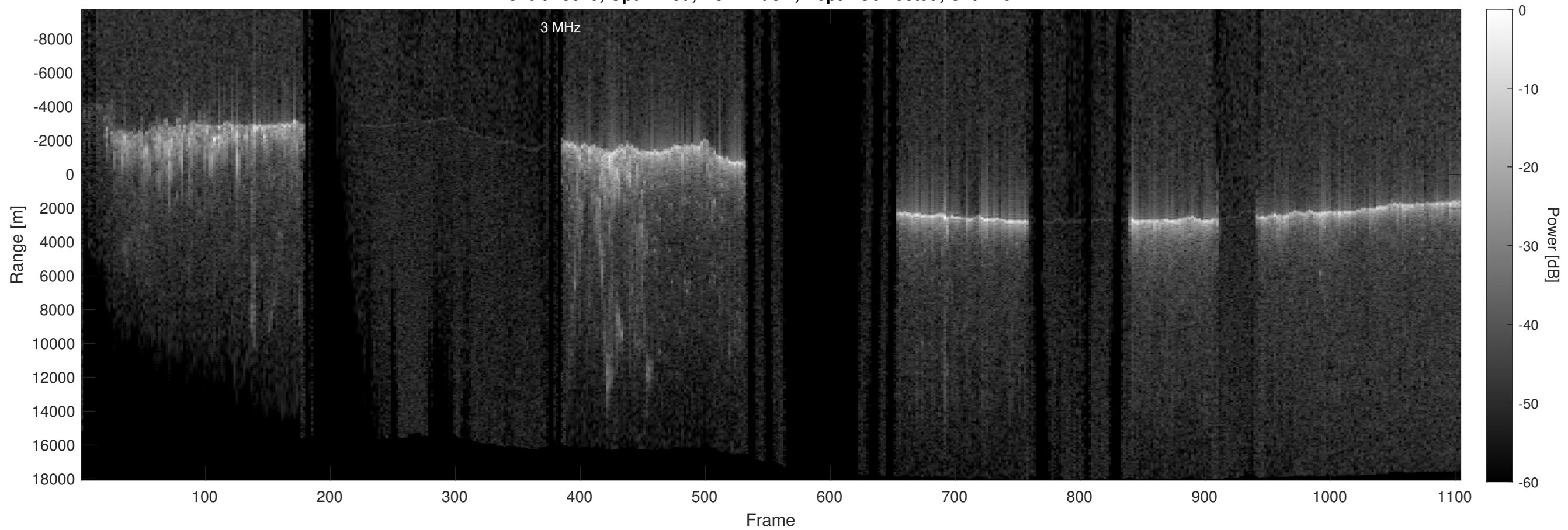
Orbit 18619, Optimized, No Window, Depth-Corrected, Channel 2
