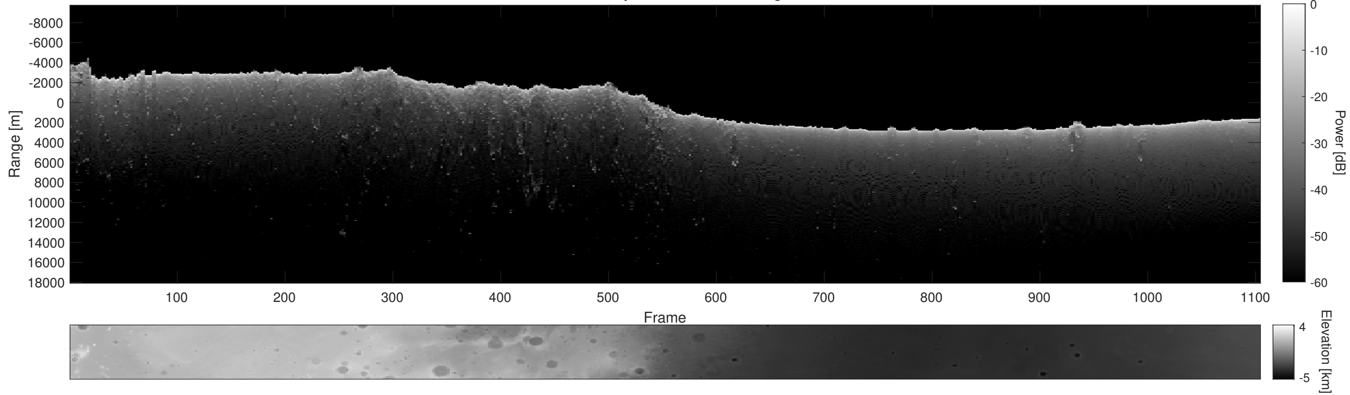
Orbit 18619, Depth-Corrected Cluttergram
