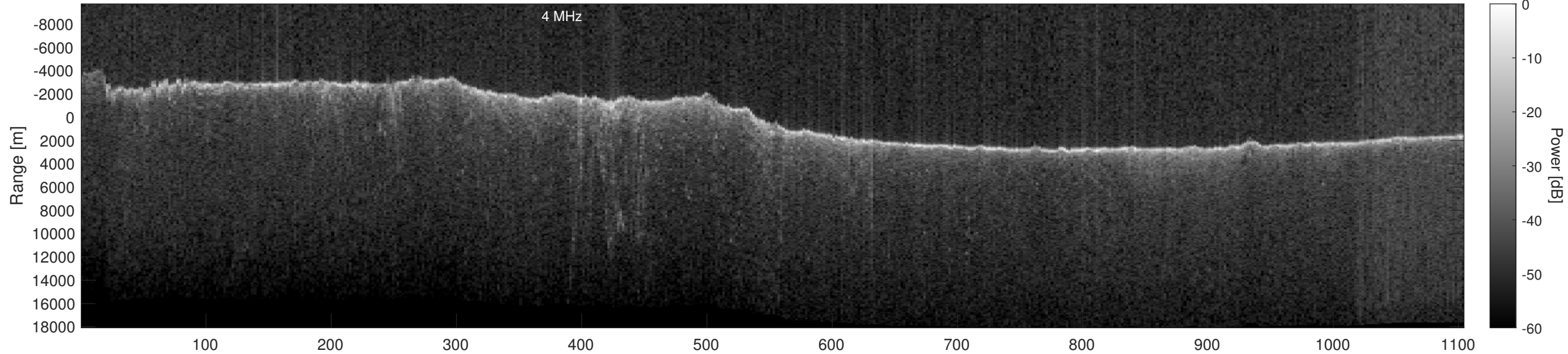
Orbit 18619, Optimized, Window, Depth-Corrected, Channel 2
