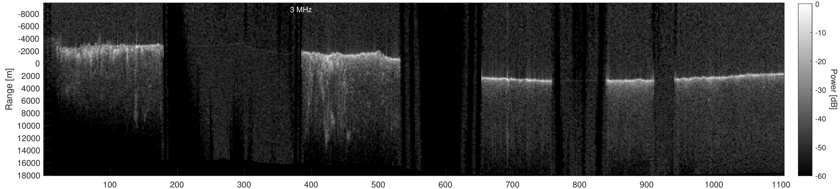
Orbit 18619, Depth-Corrected Cluttergram
