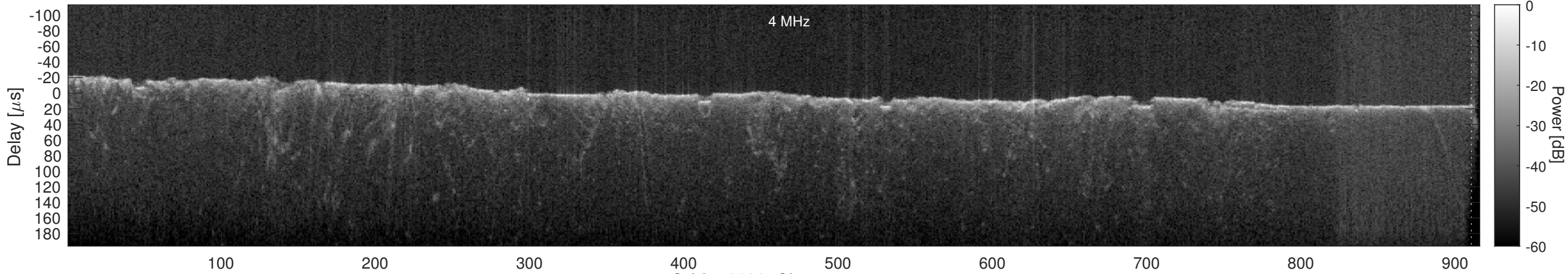
Orbit 18620, Cluttergram
