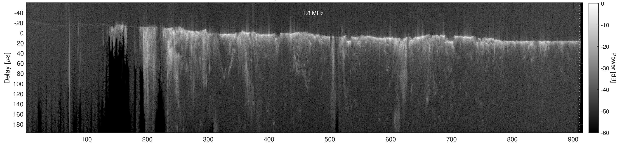
Orbit 18620, Cluttergram
