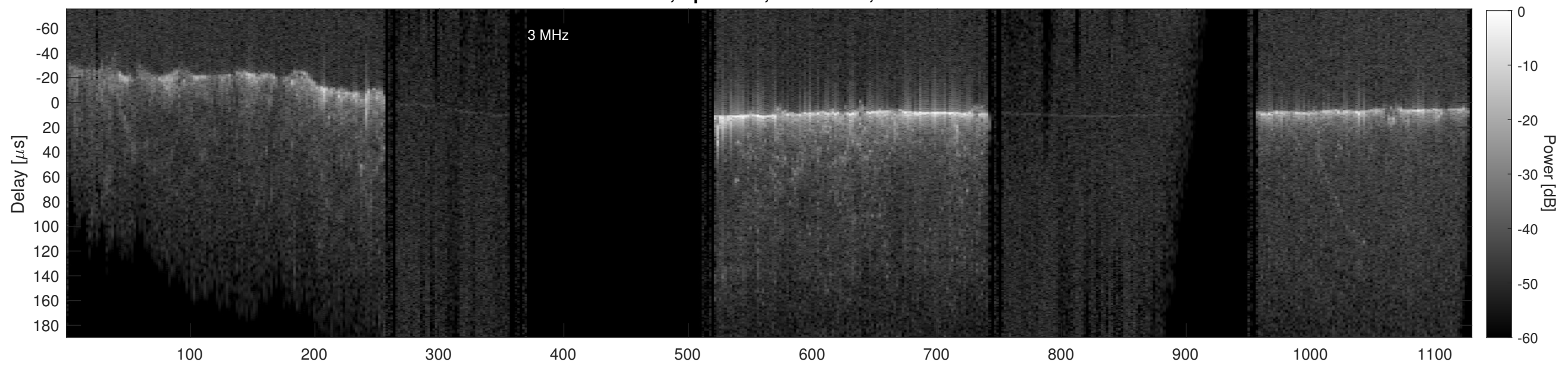
Orbit 18622, Cluttergram
