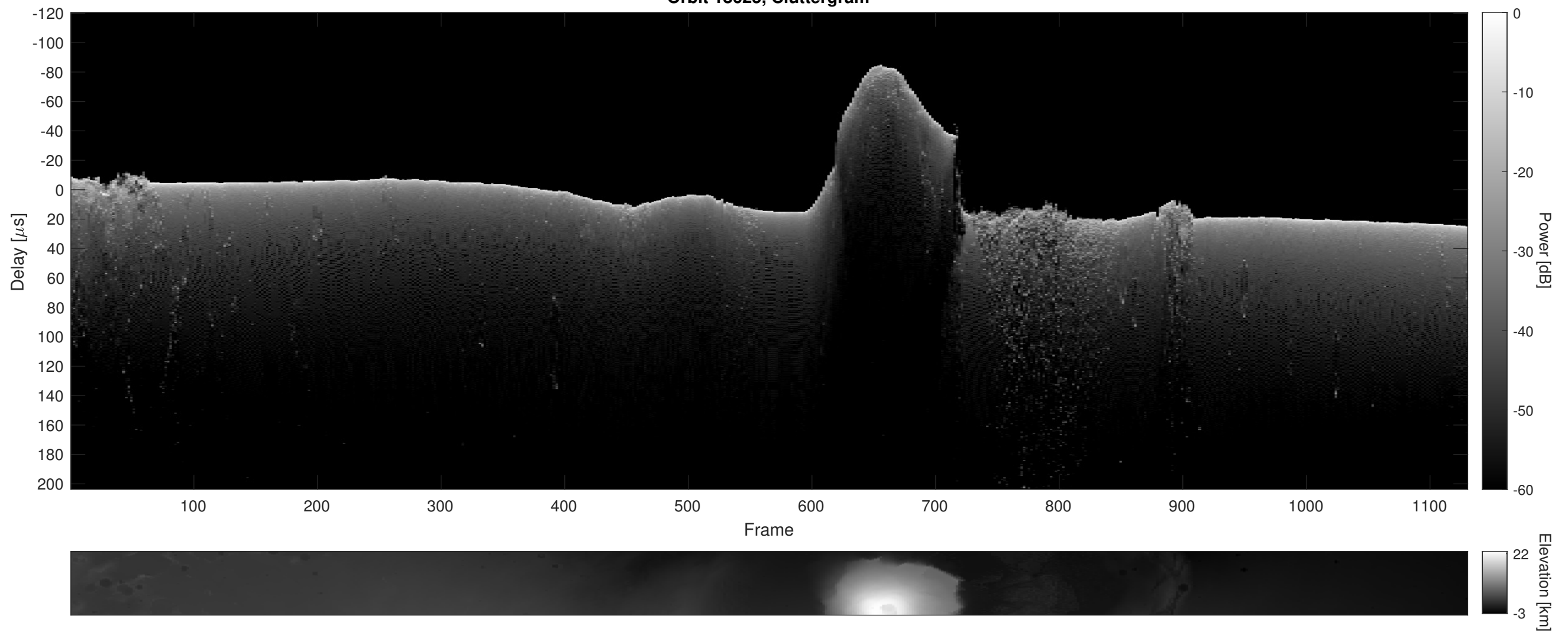
Orbit 18625, Cluttergram
