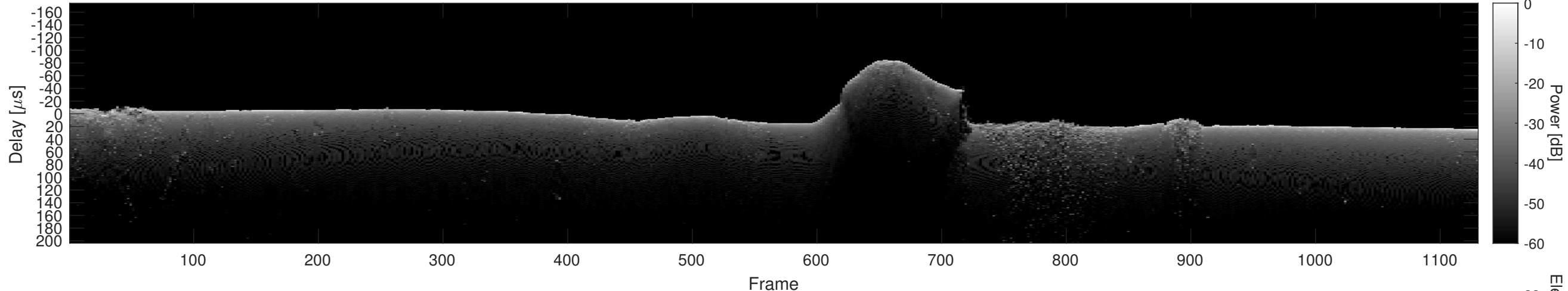
Orbit 18625, Cluttergram
