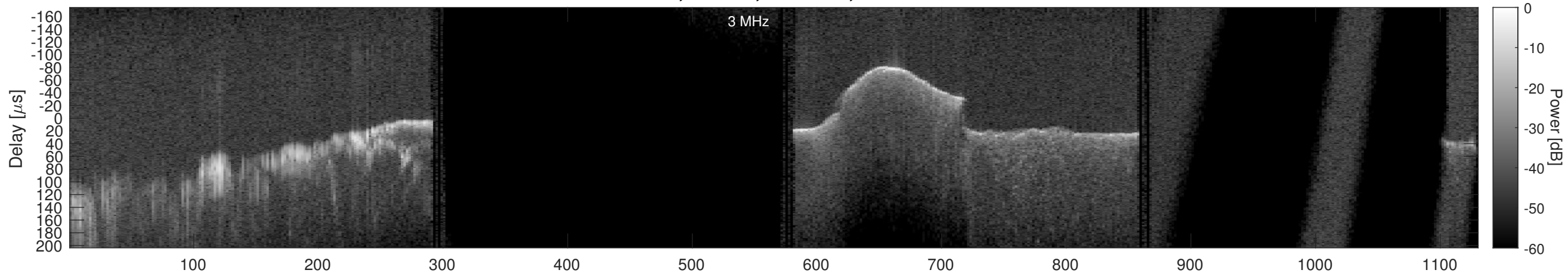
Orbit 18625, Window, Channel 2, Chapman
