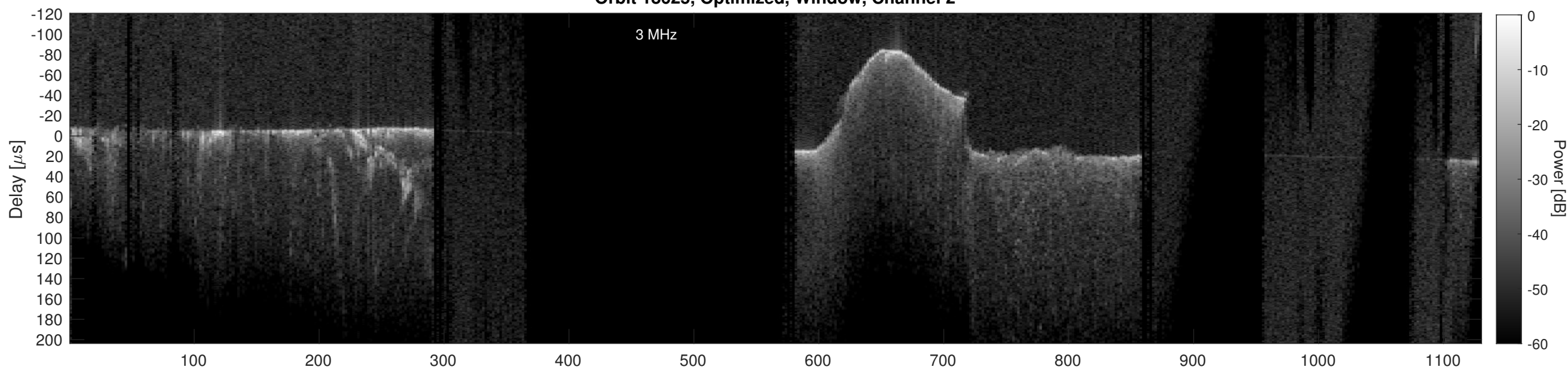
Orbit 18625, Cluttergram
