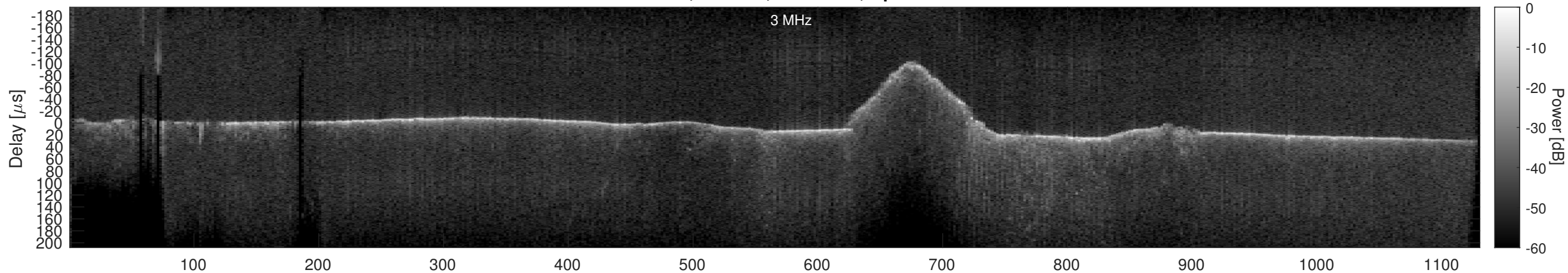
Orbit 18632, Cluttergram
