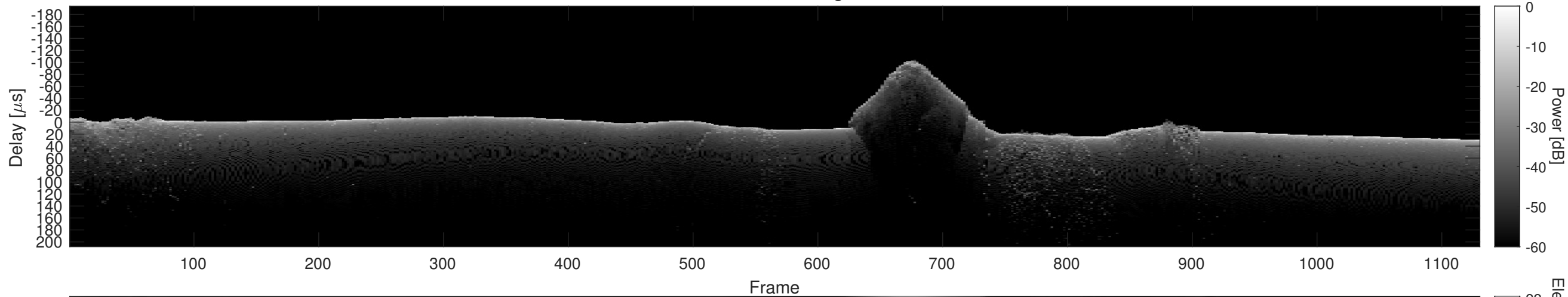
Orbit 18632, Cluttergram
