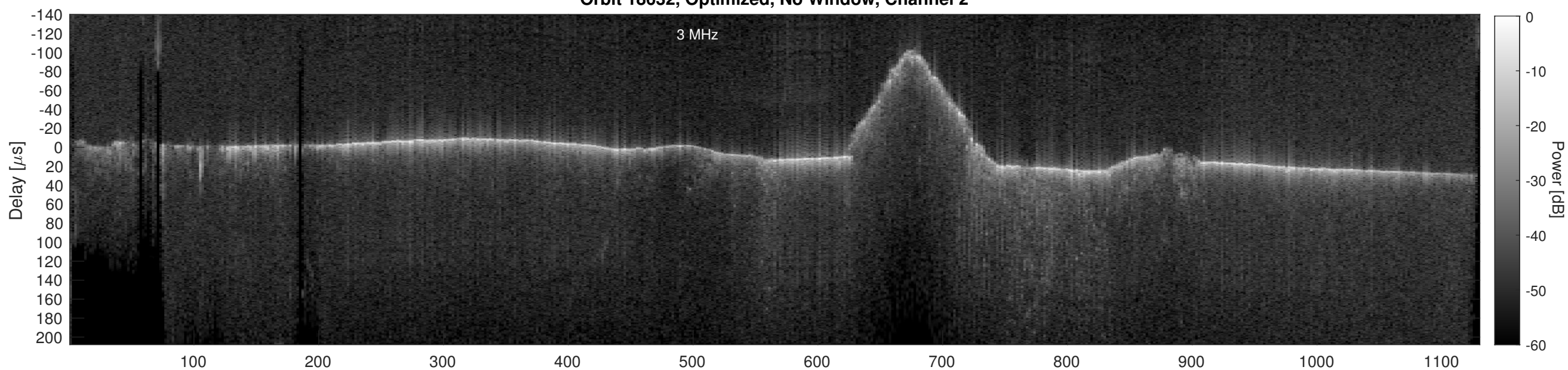
Orbit 18632, Cluttergram
