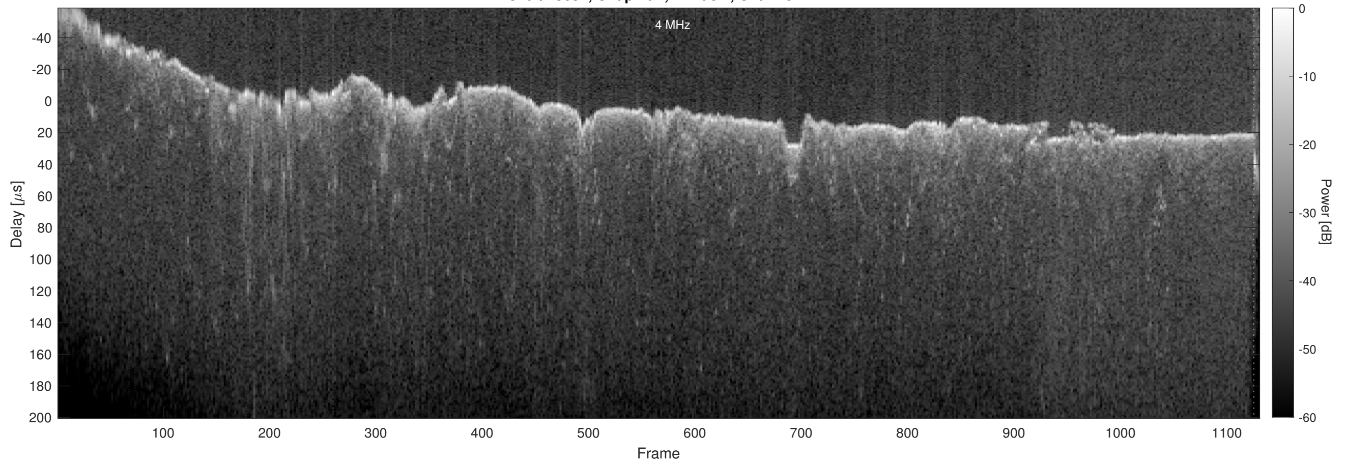
Orbit 18634, Chapman, Window, Channel 2
