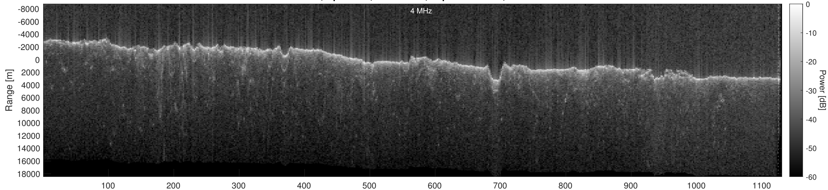
Orbit 18634, Optimized, No Window, Depth-Corrected, Channel 2
