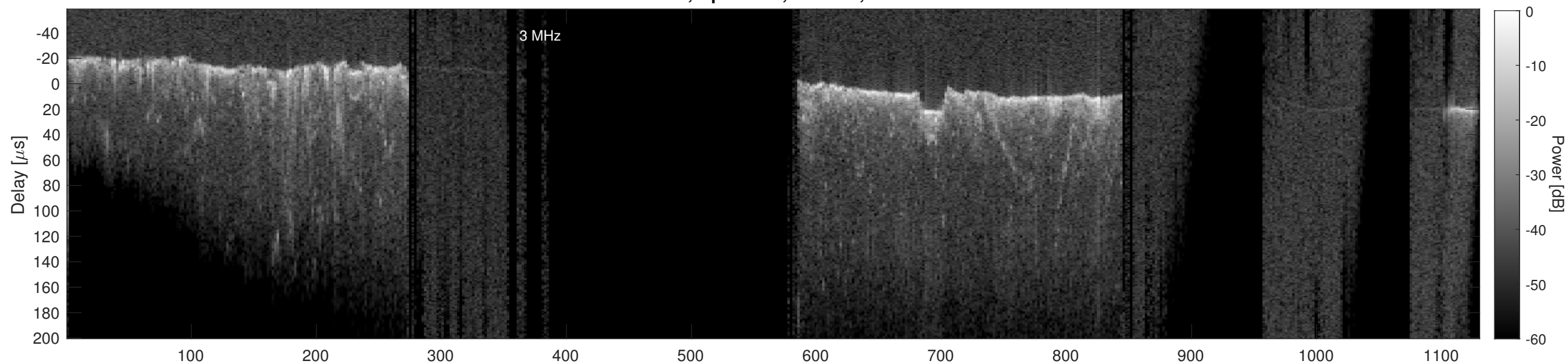
Orbit 18634, Cluttergram
