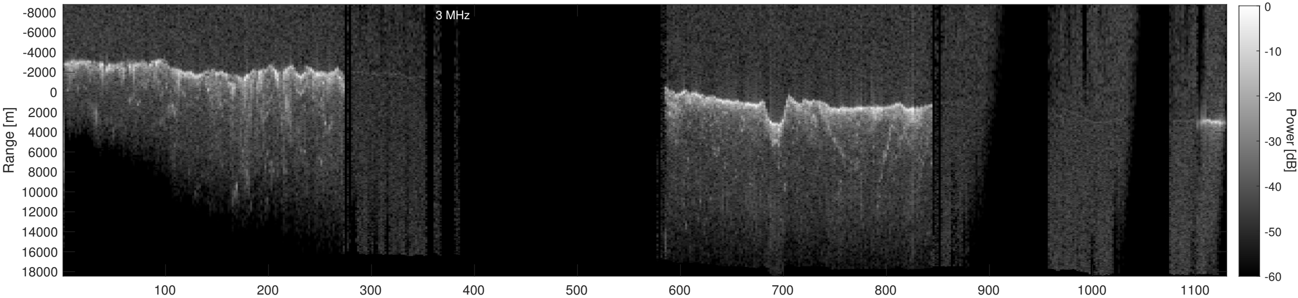
Orbit 18634, Depth-Corrected Cluttergram
