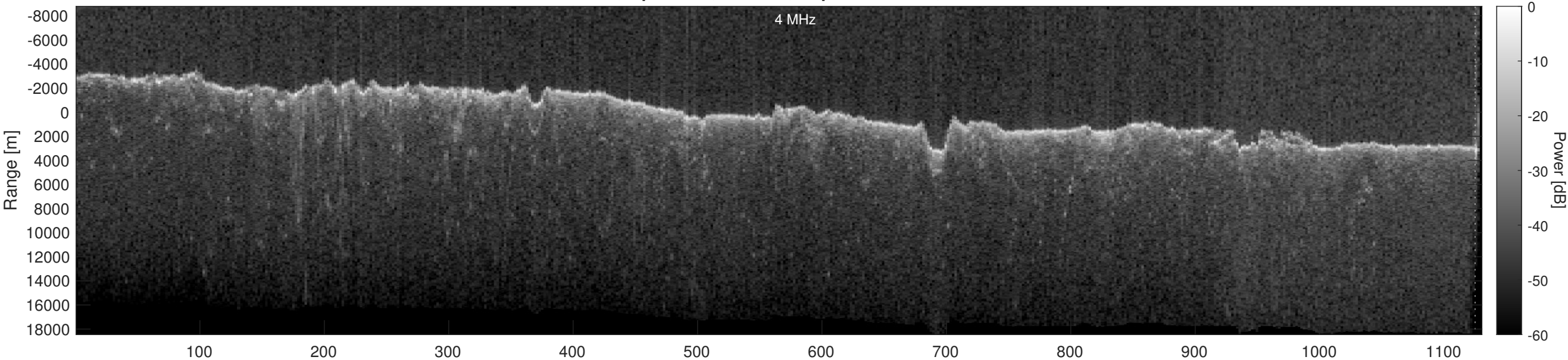
Orbit 18634, Optimized, Window, Depth-Corrected, Channel 2
