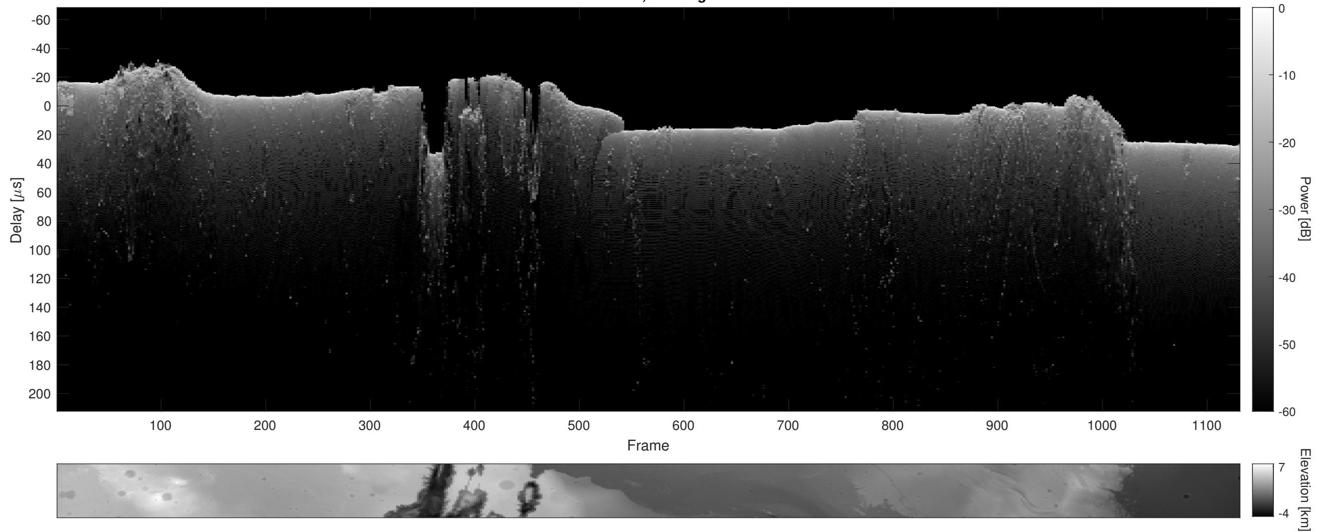
Orbit 18635, Cluttergram
