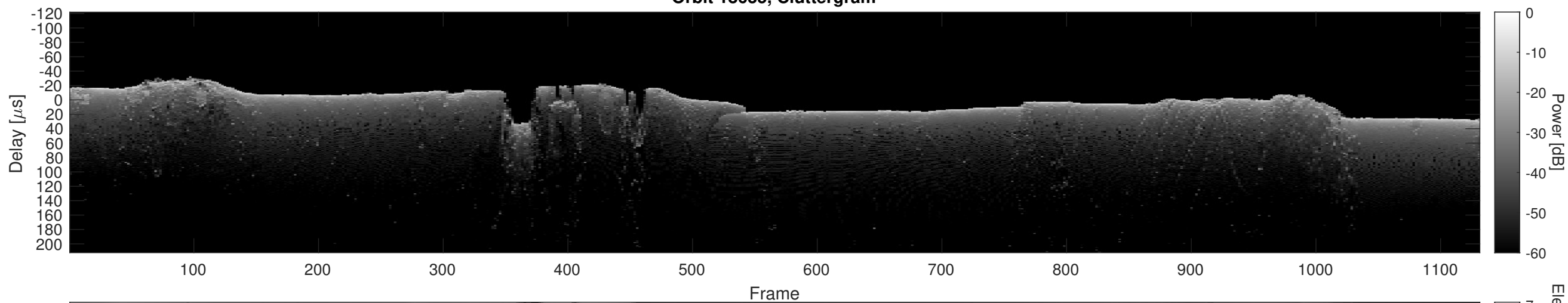
Orbit 18635, Cluttergram
