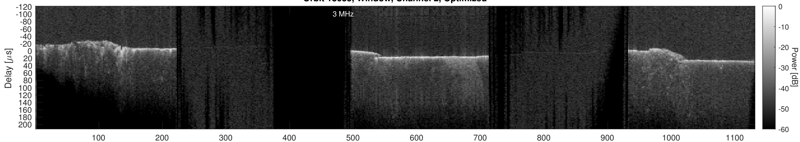
Orbit 18635, Cluttergram
