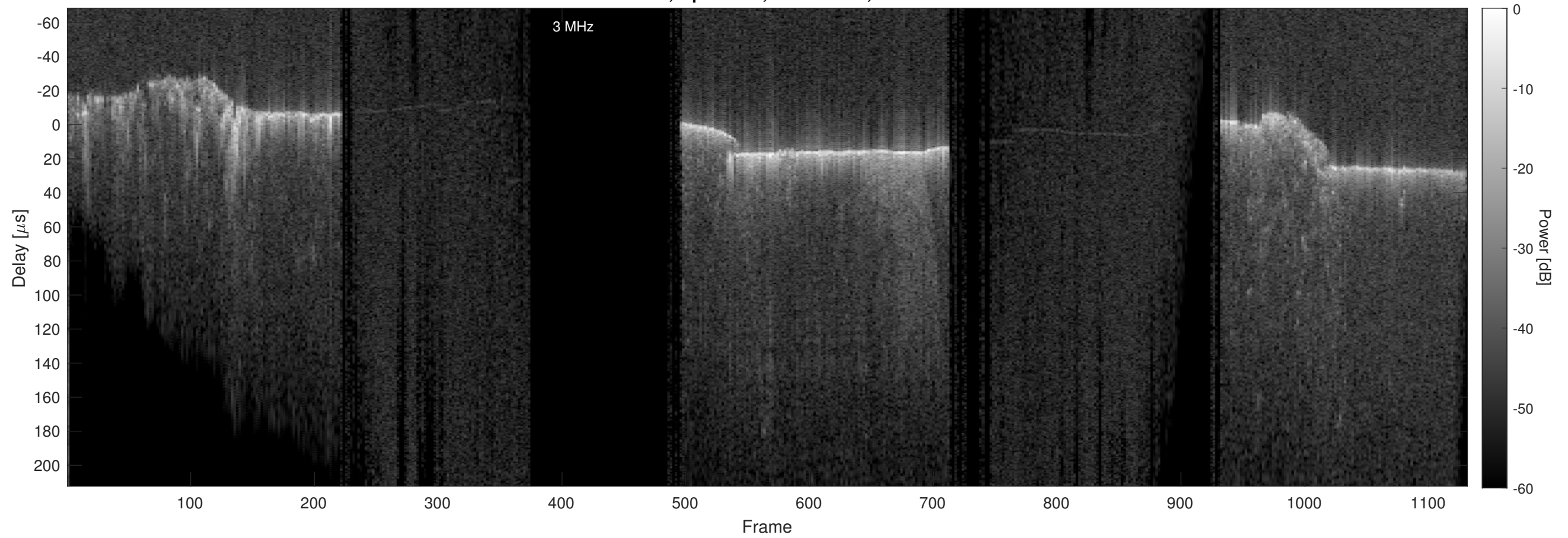
Orbit 18635, Optimized, No Window, Channel 2
