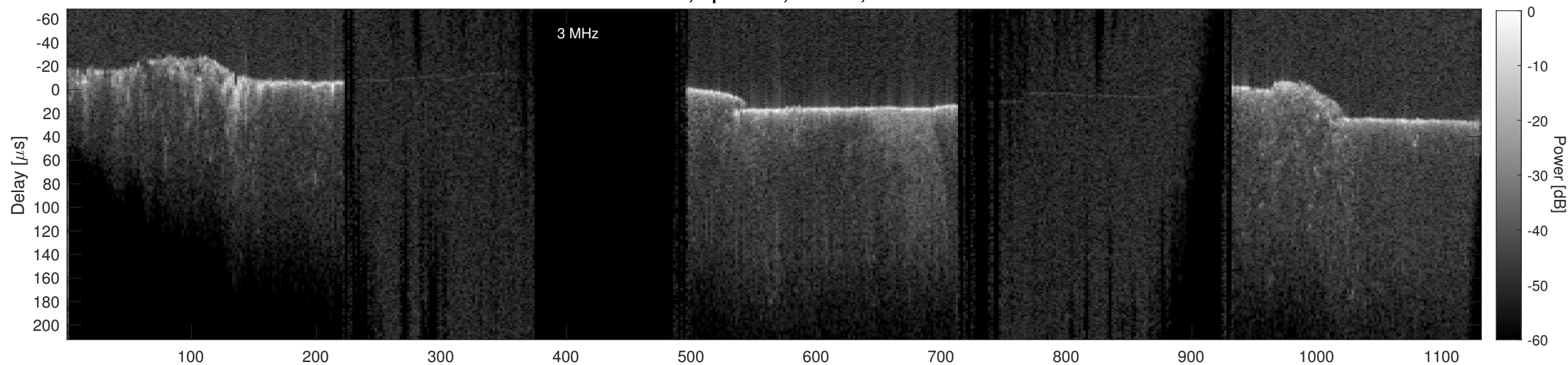
Orbit 18635, Cluttergram
