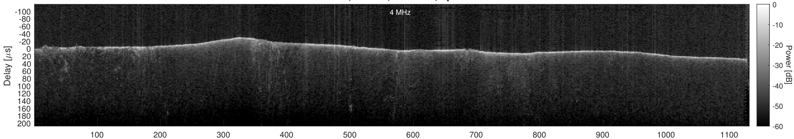
Orbit 18639, Cluttergram
