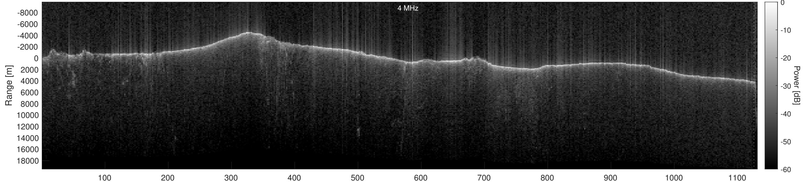
Orbit 18639, Optimized, No Window, Depth-Corrected, Channel 2
