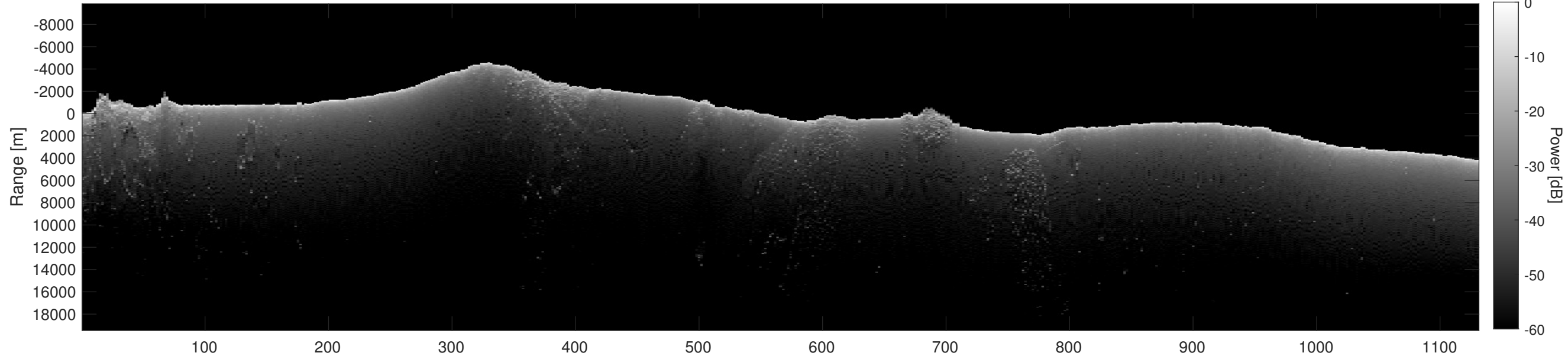
Orbit 18639, Depth-Corrected Cluttergram
