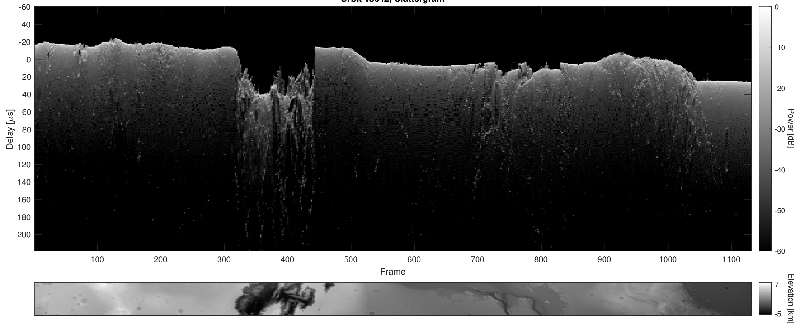
Orbit 18642, Cluttergram
