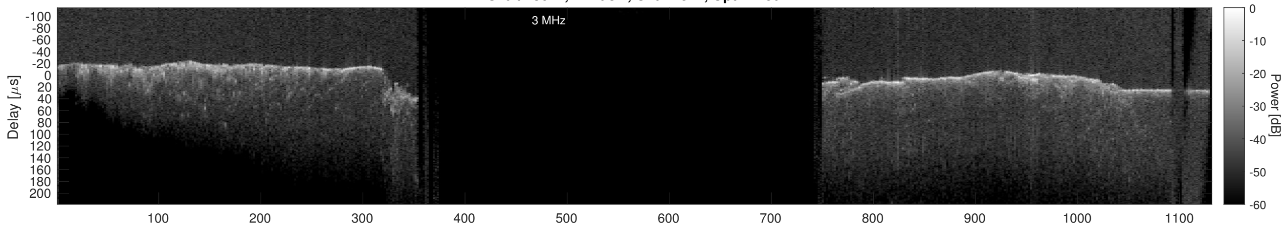
Orbit 18642, Cluttergram
