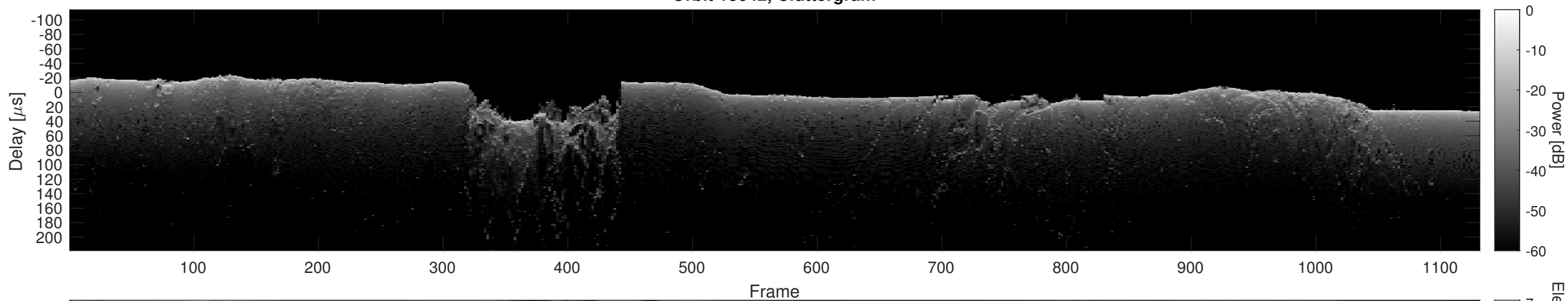
Orbit 18642, Cluttergram
