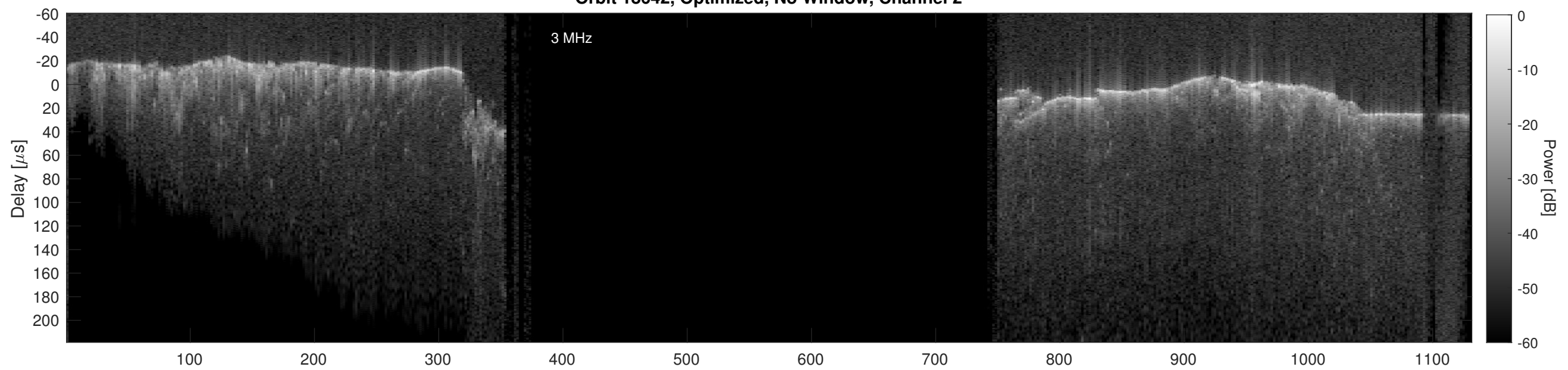
Orbit 18642, Cluttergram
