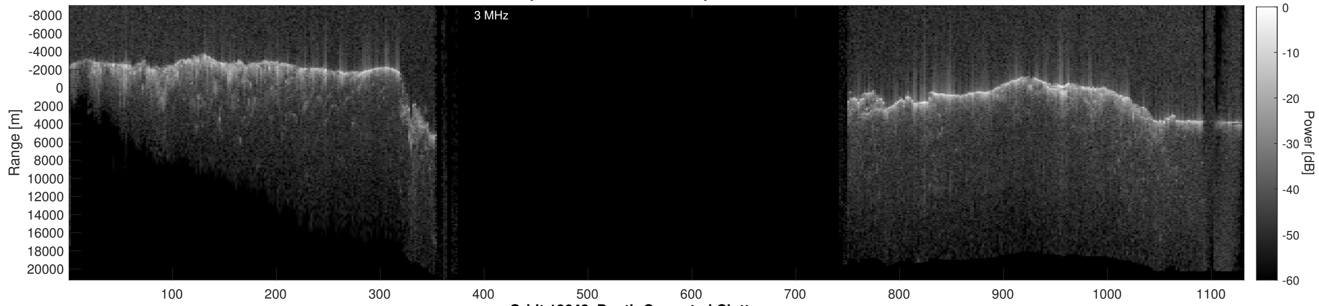
Orbit 18642, Depth-Corrected Cluttergram
